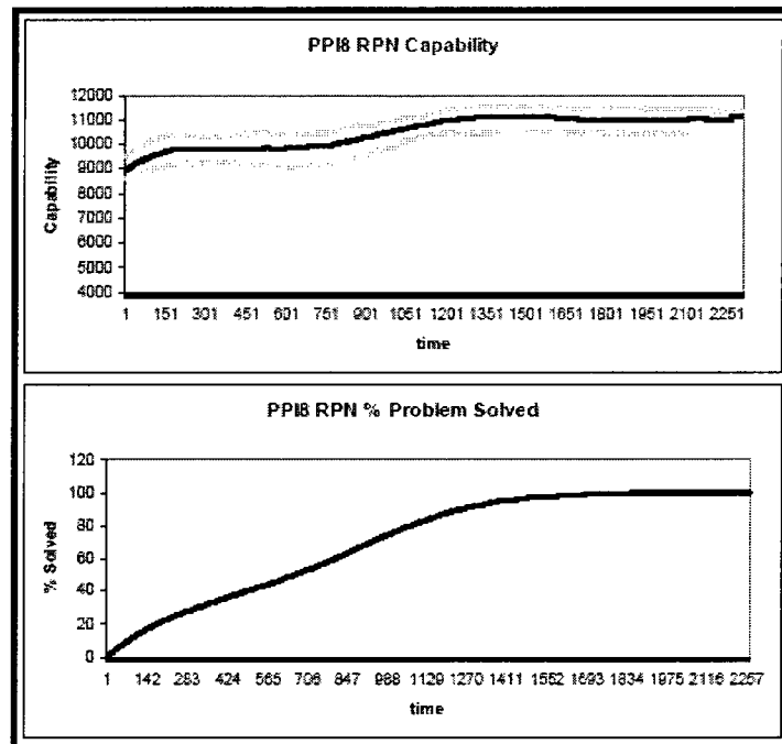
Figure 32. PPI8 patterns
