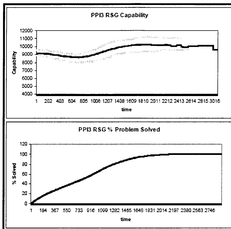
Figure 27. PPI3 patterns
